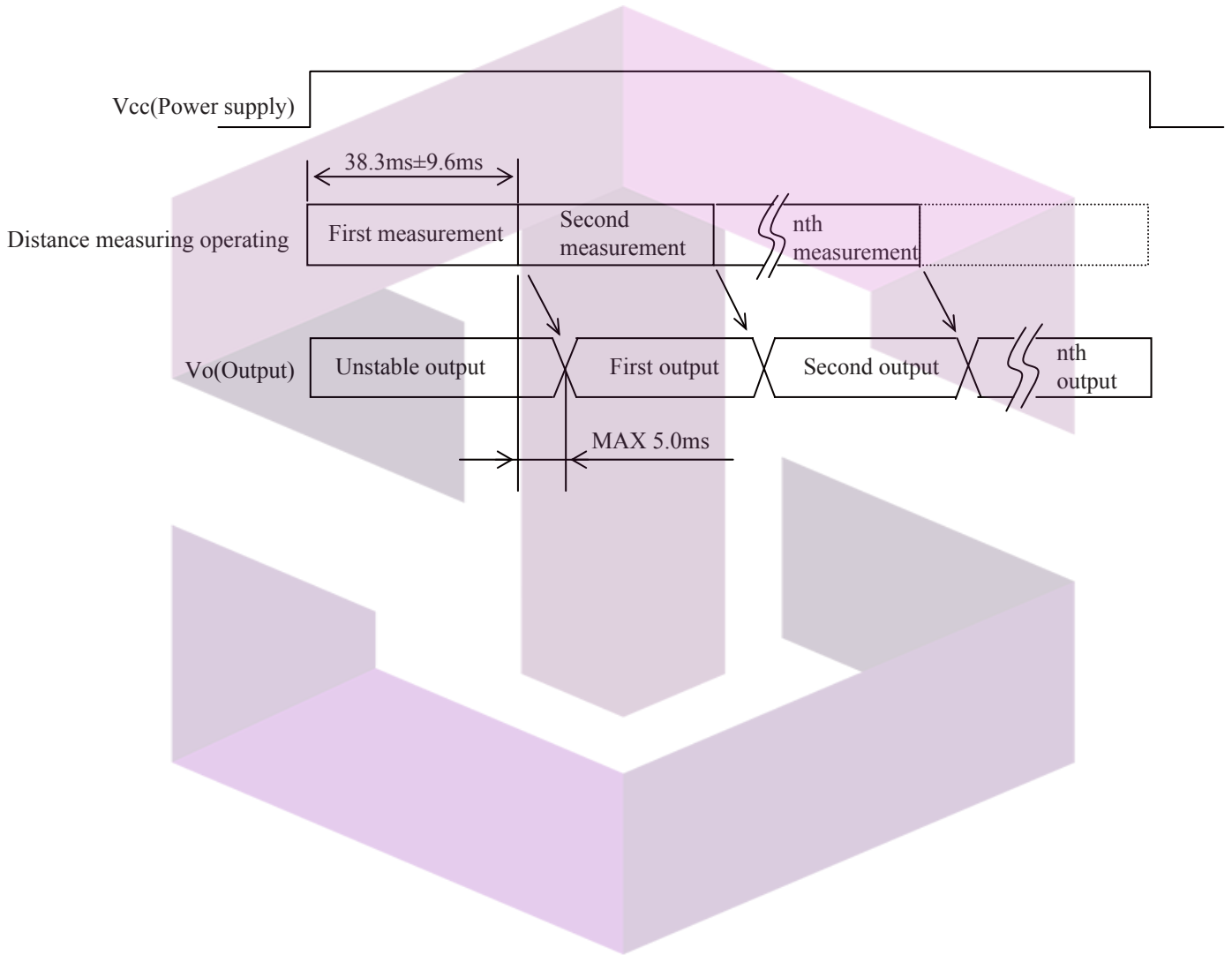
Fig. 1 Timing chart
